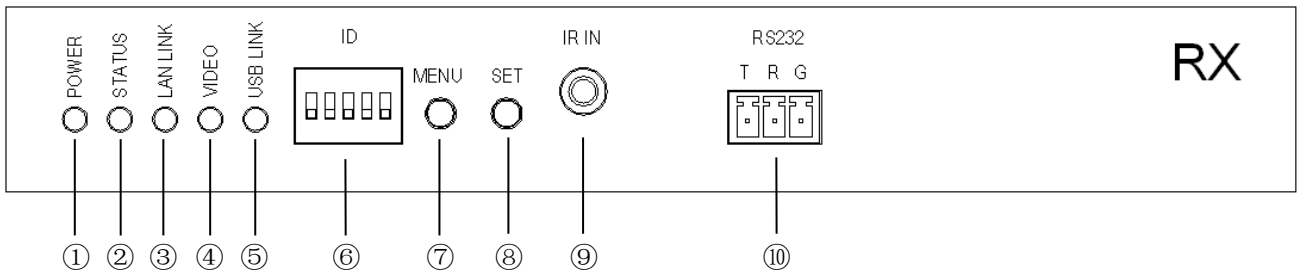
Picture 1.2 Front panel of Receiver (RX)
